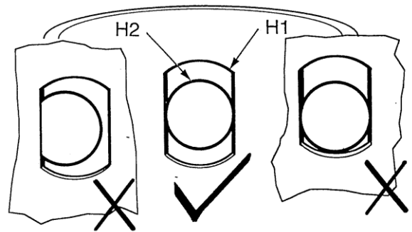
fig SP4: clamp band alignment
